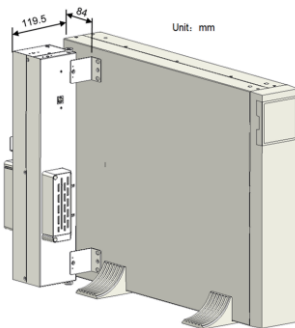
Left position
