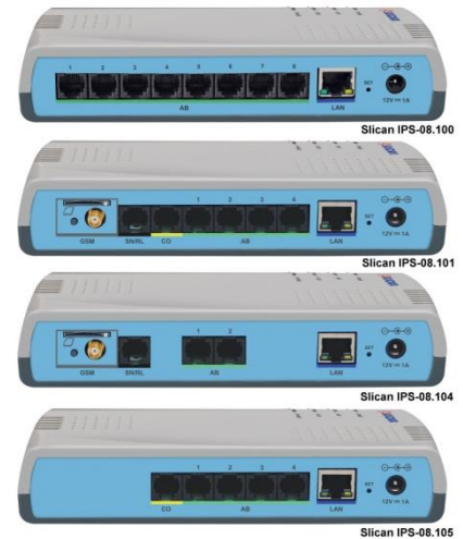
centrala IPS-08
