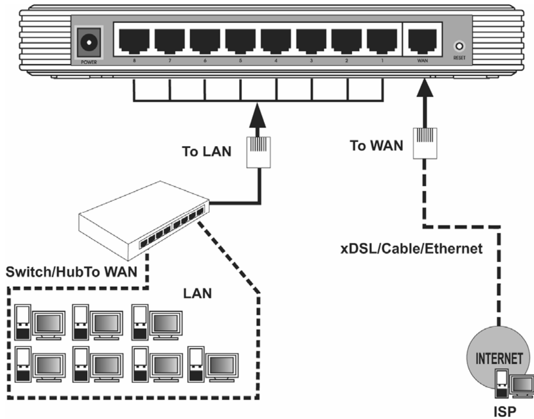
Figure 2-1 Hardware Installation of the TL-R860 Cable/DSL Router
